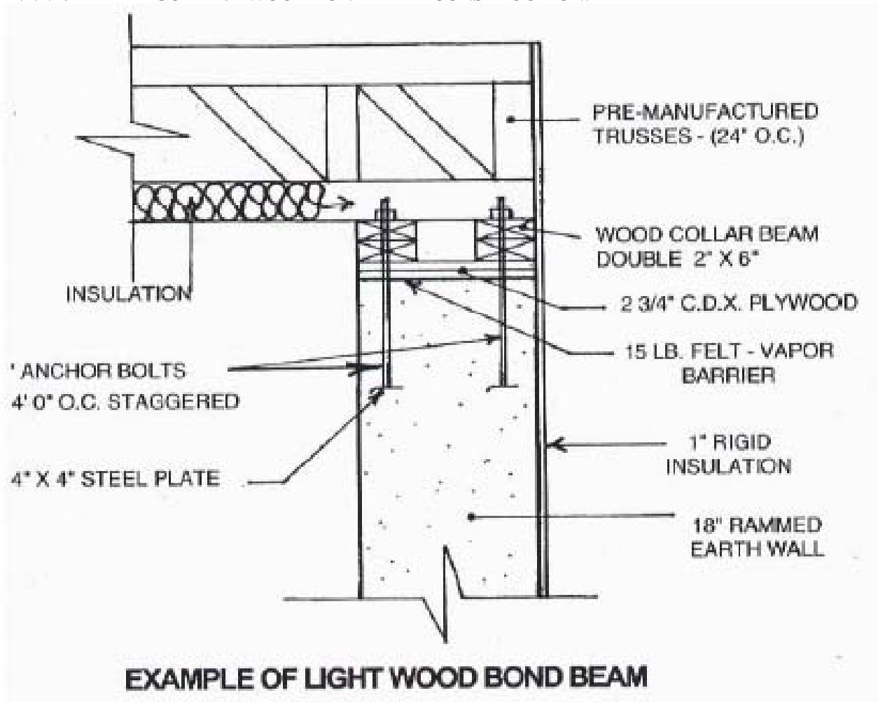
14.7.4.40 FIGURE 10 - WOOD BOND BEAM CONSTRUCTION:
