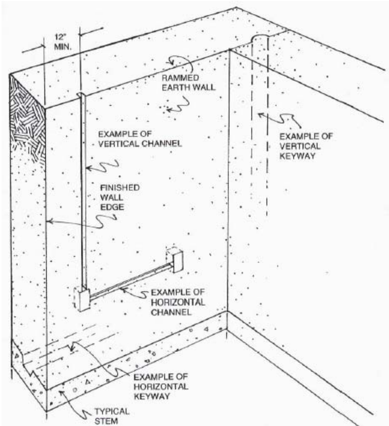
14.7.4.31 FIGURE 2 - CHANNEL
