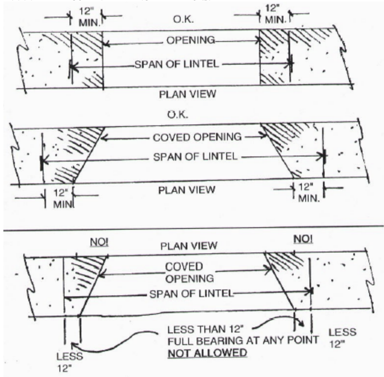
14.7.4.45 FIGURE 15 - BEARING LIMITATIONS:
