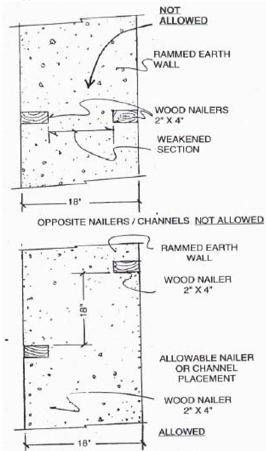
FIGURE 4 - NAILER:
